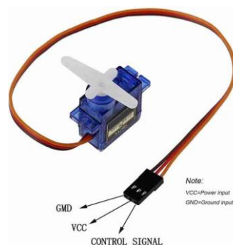
Gambar 3. Motor Servo
